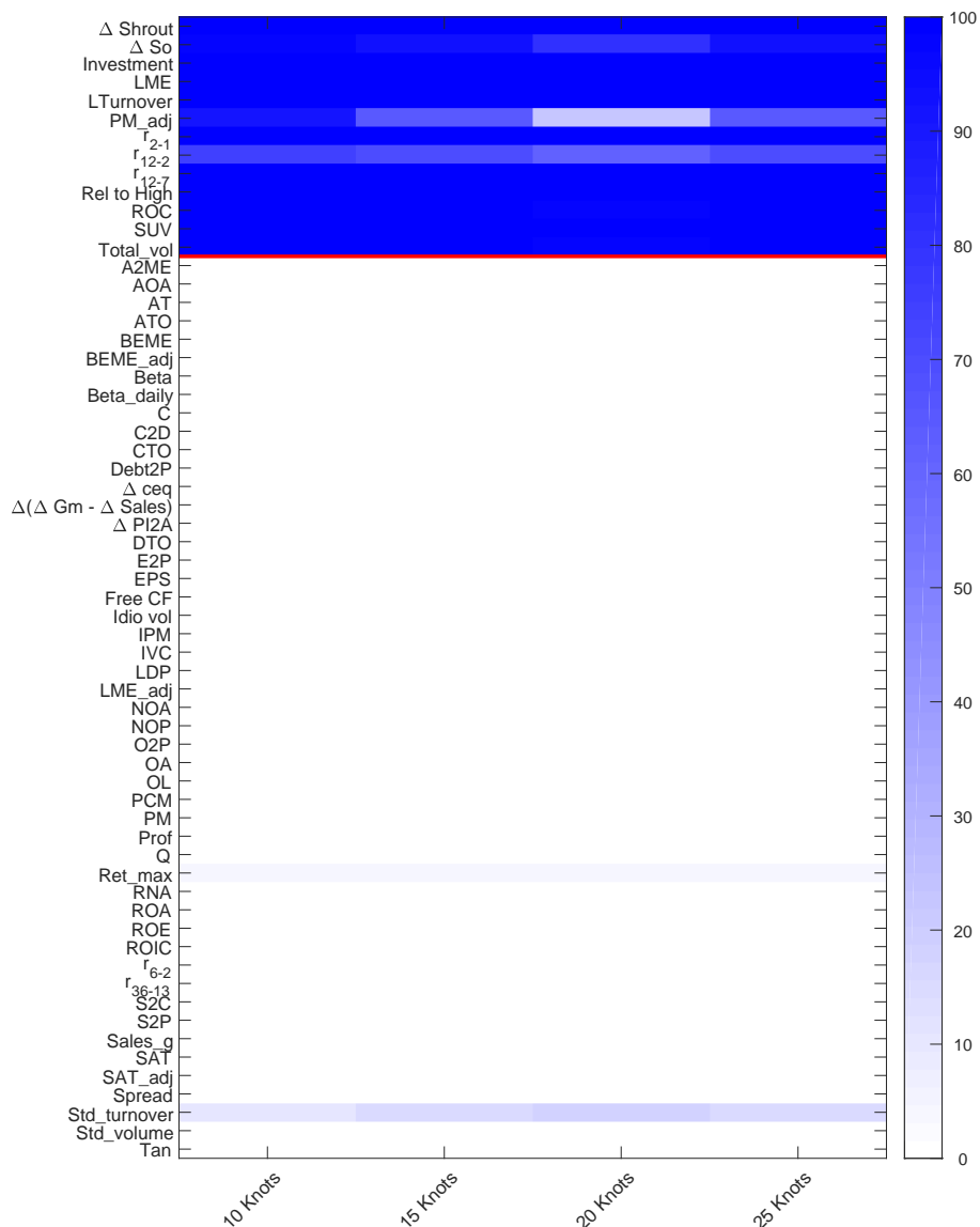
Figure A.5: Selected Characteristics in Simulations: Empirical Data-Generating Process (different Knot Numbers)
