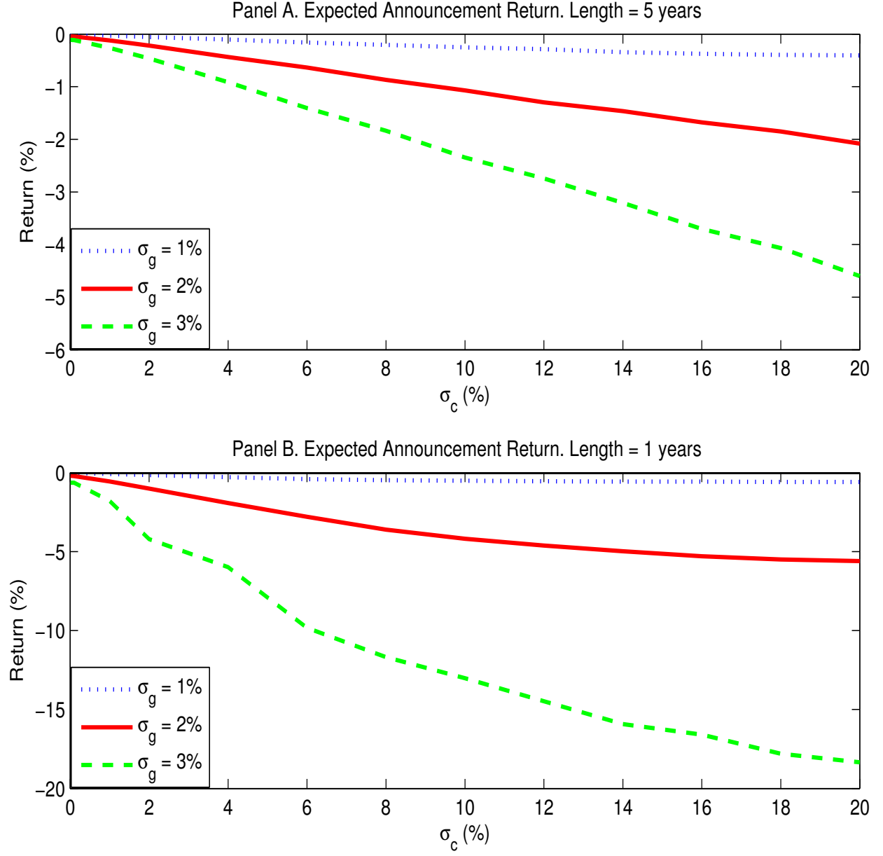
Figure 7. Expected announcement return and the downturn length. This figure plots the expectation of the announcement return R(\hat{g}_\tau) , which is the instantaneous stock return at the announcement of a policy change at time \tau . The expectation integrates out uncertainty about \hat{g}_\tau as perceived at the beginning of the downturn, as well as uncertainty about c conditional on the policy being changed. The downturn length is \tau - t_0 = 5 years in Panel A and 1 year in Panel B. We vary \sigma_g and \sigma_c , and all other parameters are from Table 1.
