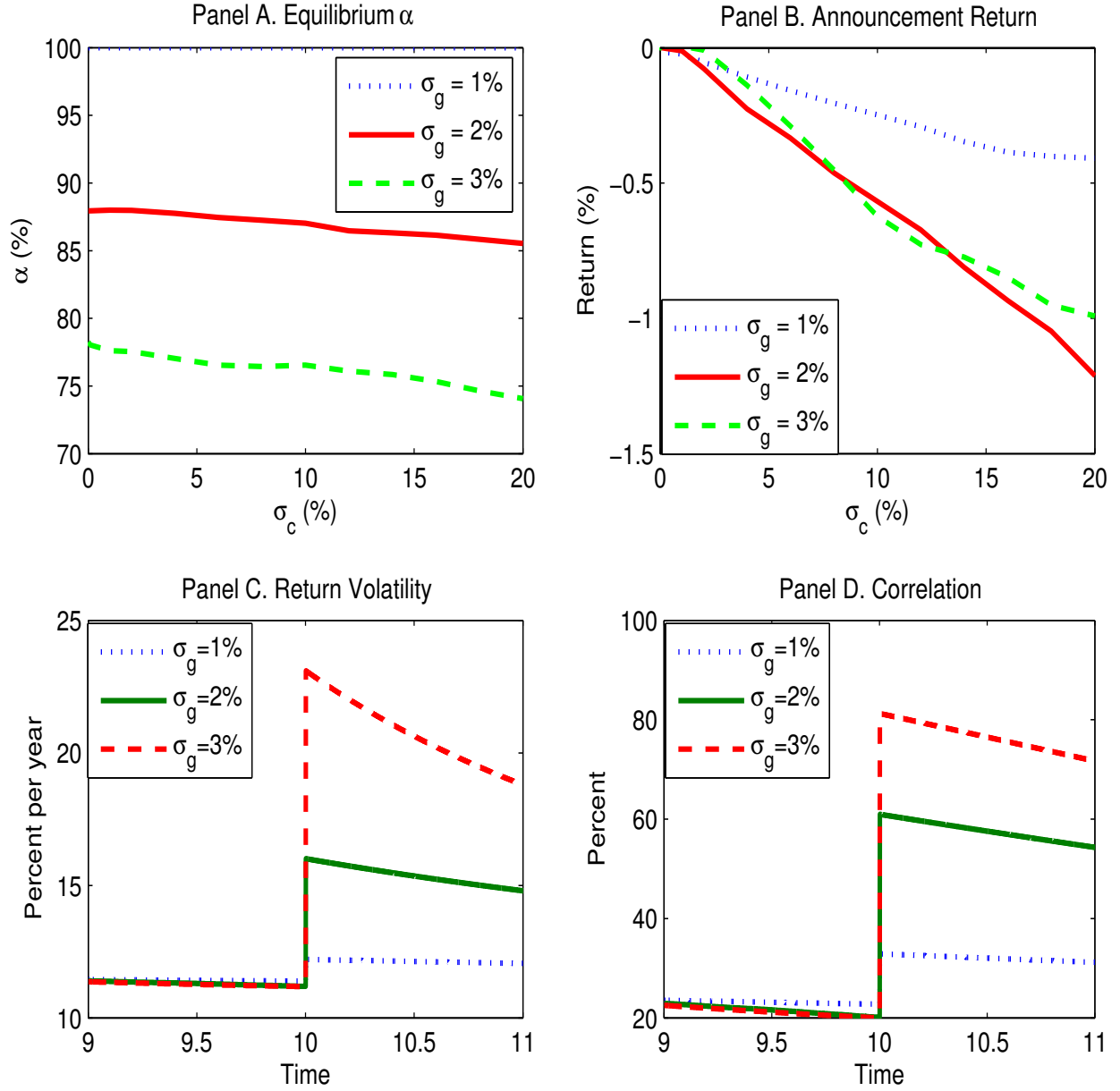
Figure 14. Investment adjustment. This figure plots the results from the extension of the benchmark model in which firms can disinvest at time \tau . Panel A plots the equilibrium fraction of firms that choose to remain invested in the risky technology after the policy change. Panel B plots the corresponding stock return expected at the announcement of a policy change. Panels C and D plot the expected dynamics of \sigma_{M,t} and \rho_t , respectively, around a policy change at time \tau = 10 . The parameters are in Table 1, except that \mu = 0.02 (we reduce \mu from its benchmark value to obtain \alpha < 1 in equilibrium) and \sigma_g takes three different values, 1%, 2%, and 3% per year. The downturn length is set to 5 years in all four panels.
