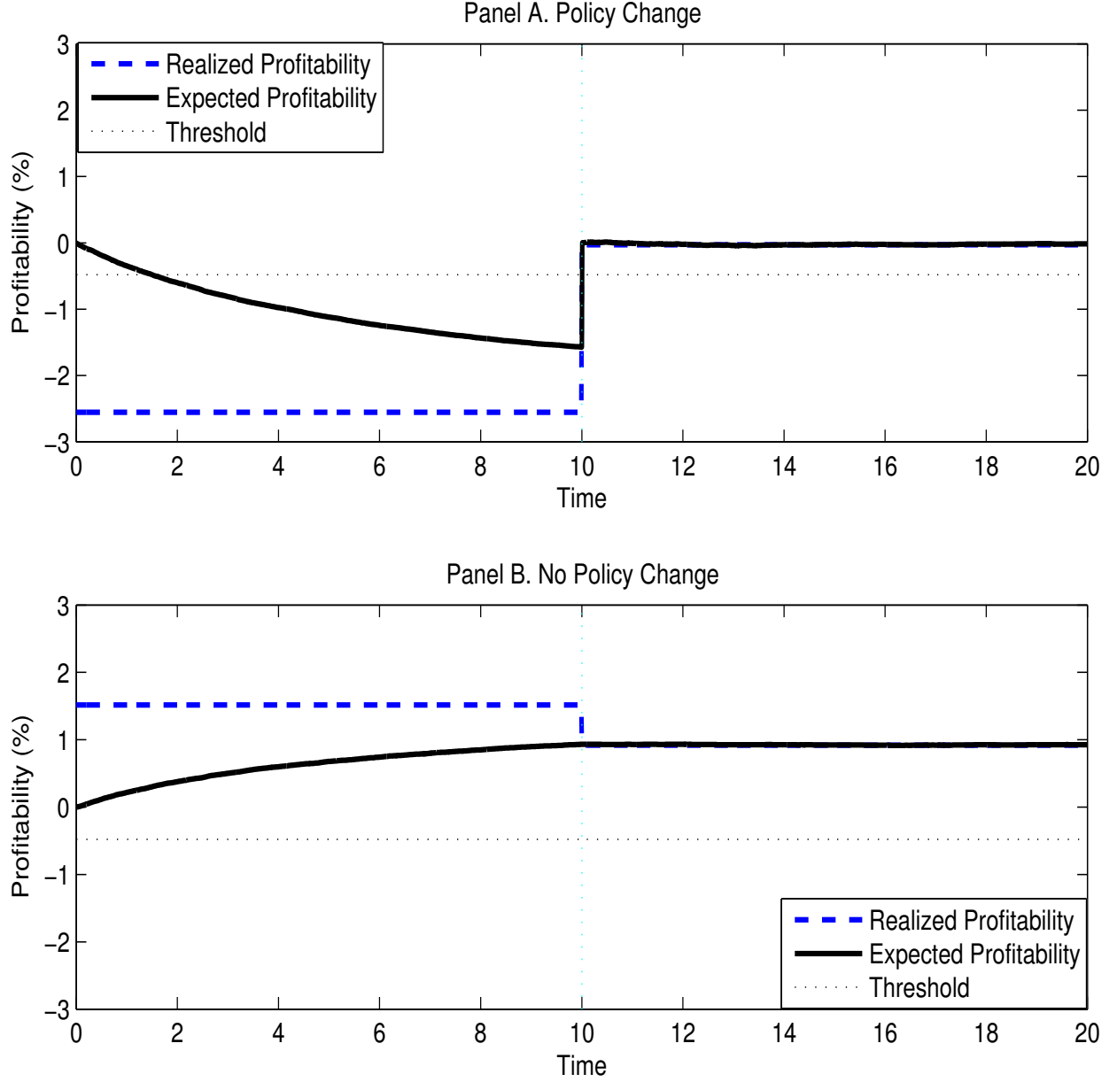
Figure 1. Profitability dynamics and the policy decision. This figure plots the expected dynamics of \hat{g}_t (solid line) and realized profitability (dashed line) under the parameter values from Table 1. Realized profitability is the average profitability across all firms, plotted in excess of \mu so that its unconditional mean is zero. The figure also plots the threshold \underline{g}(c) (dotted line). All three lines are average paths across many simulated samples. The top panel averages across the samples in which a policy change occurred at time \tau = 10 , whereas the bottom panel conditions on no policy change.
