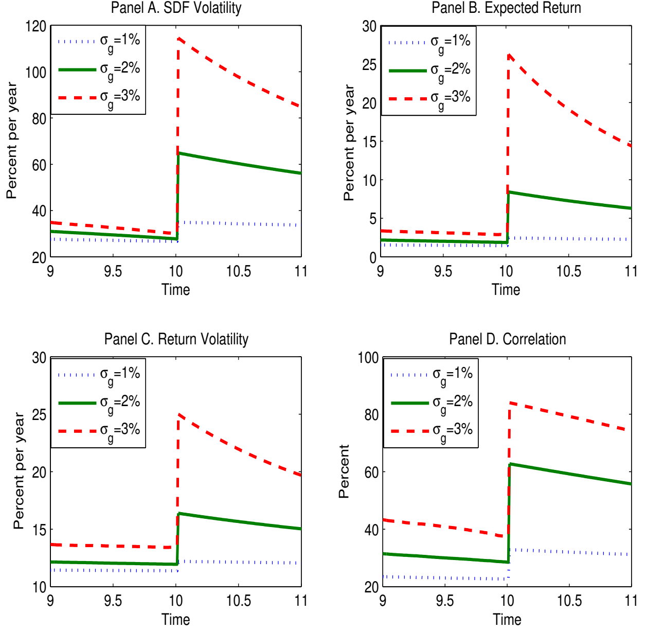
Figure 10. Properties of returns around policy decisions that result in a policy change. This figure plots the expected dynamics of the volatility of the stochastic discount factor, \sigma_{\pi,t} (Panel A), the conditional expected stock market return, \mu_{M,t} (Panel B), the conditional volatility of stock market returns, \sigma_{M,t} (Panel C), and the pairwise correlation between stocks, \rho_t (Panel D), all conditional on a policy change at time \tau = 10 . The jump-related components at time \tau are not plotted. The downturn length is \tau - t_0 = 5 years, so that \hat{g}_5 = 0 . The parameters are in Table 1, except for \sigma_g , which takes three different values, 1%, 2%, and 3% per year.
