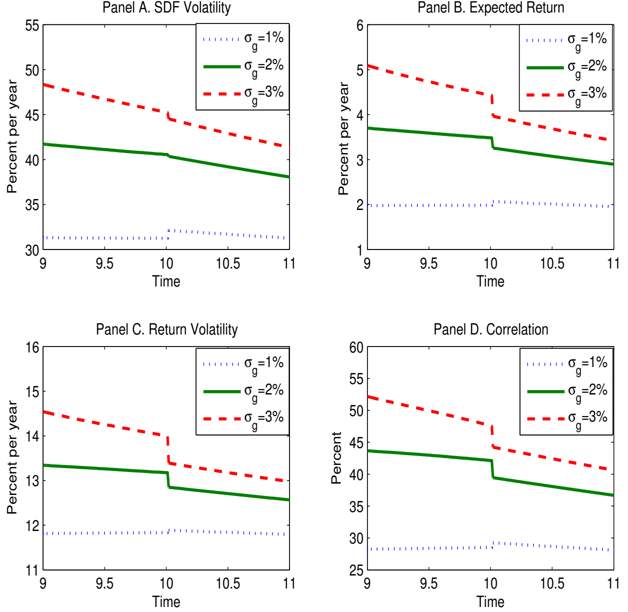
Figure 11. Properties of returns around policy decisions that result in no policy change. This figure plots the expected dynamics of the volatility of the stochastic discount factor, \sigma_{\pi,t} (Panel A), the conditional expected stock market return, \mu_{M,t} (Panel B), the conditional volatility of stock market returns, \sigma_{M,t} (Panel C), and the pairwise correlation between stocks, \rho_t (Panel D), all conditional on no policy change at time \tau = 10 . The jump-related components at time \tau are not plotted. The downturn length is \tau - t_0 = 5 years, so that \hat{g}_5 = 0 . The parameters are in Table 1, except for \sigma_g , which takes three different values, 1%, 2%, and 3% per year.
