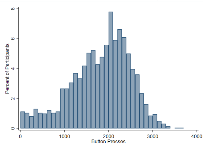
Figure 4d. 2018 Extra Card Coding Task
