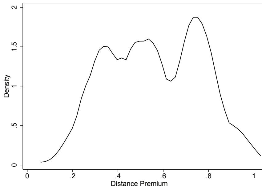
Figure 2: Distance premium, by 6-digit industry
