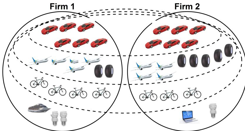
Figure 4: Incidental Merger Example
