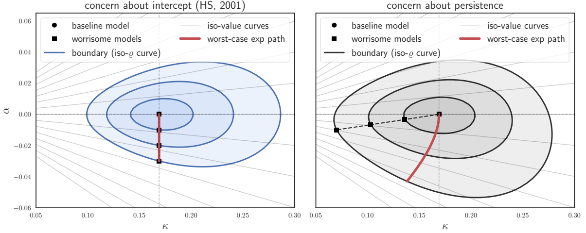
Figure 2: Iso- \rho and iso-value curves in the parametric class indexed by (\alpha, \kappa) for different twisting functions. The locus of points of tangency between these curves shows worst-case models for a sequence of constant \xi (left) and for a sequence of state-dependent \xi (right). Baseline model parameters are (\hat{\alpha}, \hat{\kappa}, \sigma) = (0, 0.169, 0.195) , the policy is (\bar{\alpha}_c, \bar{\beta}) = (0.499, 1) . We evaluate the iso- \rho and iso-value curves using X_0 = 0 as the initial state. The dash-dotted line denotes worrisome models as convex combinations of the baseline and (\tilde{\alpha}, \tilde{\kappa}) = (-0.01, 0.07) models.
