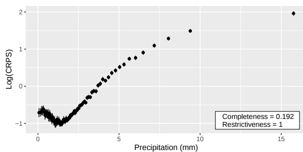
(b) log(CRPS) vs. precipitation
