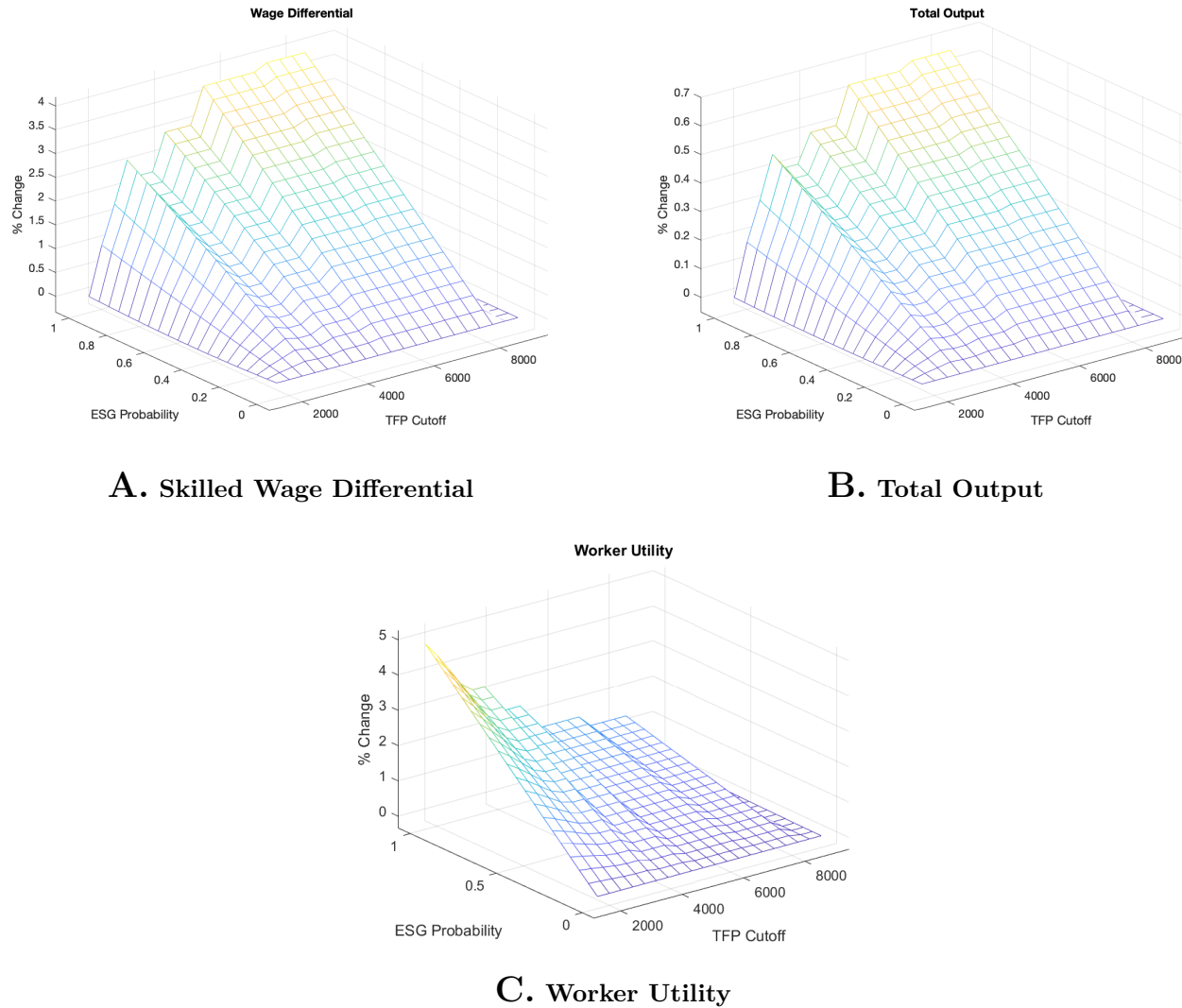
FIGURE 5. Model Counterfactuals
