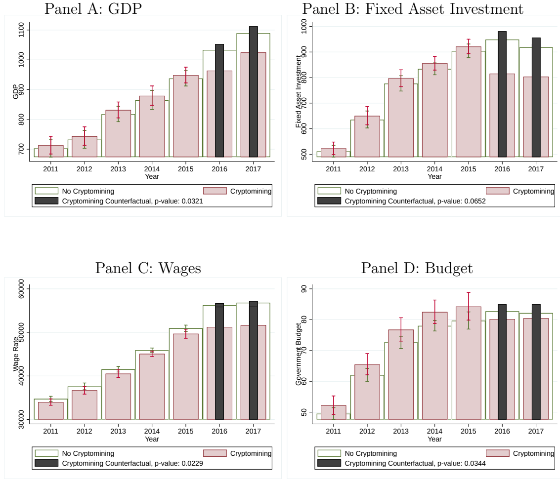
Figure 11: PARALLEL TRENDS
