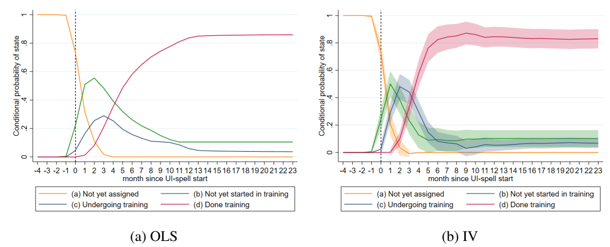
Figure 5: Training-State Probabilities
