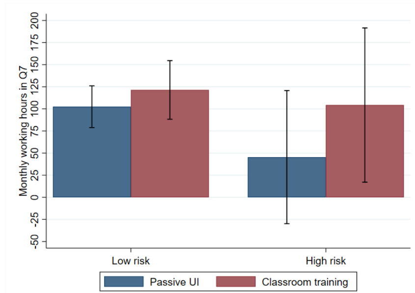
Figure 10: Policy Counterfactuals
