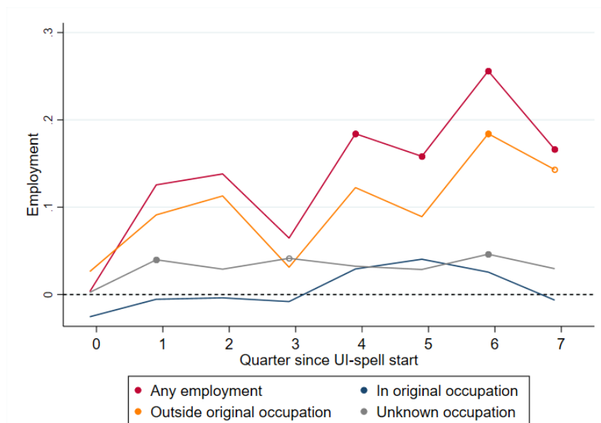
Figure 7: Occupational Mobility
