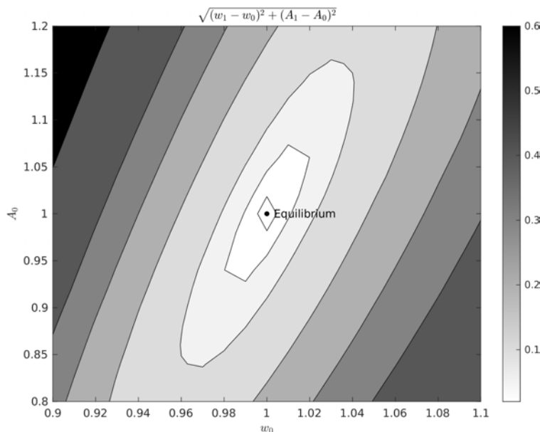
Figure A6: Norm of implied difference between (w_0, A_0) and (w_1, A_1)
