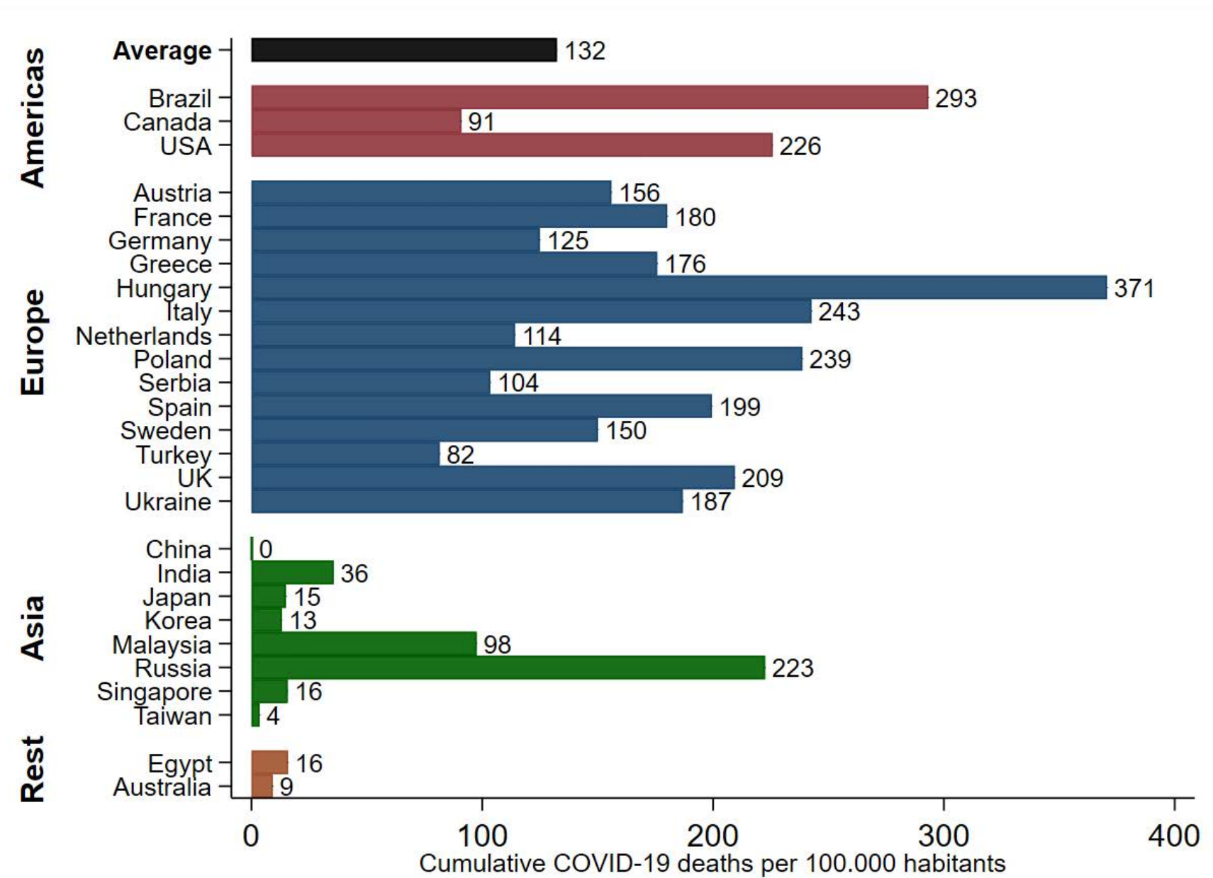
Figure A.4. Cumulative reported COVID-19 Deaths per Capita by Country
