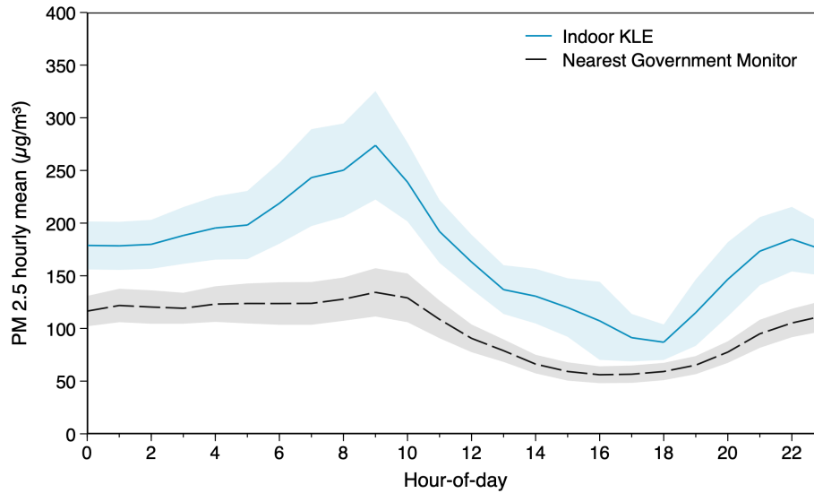
Figure A8A. Indoor PM 2.5 pattern in a single high SES household in February 2020
