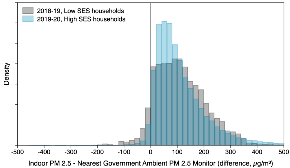
Figure A6. Indoor - Outdoor, Ambient PM 2.5 differences in low and high SES households
