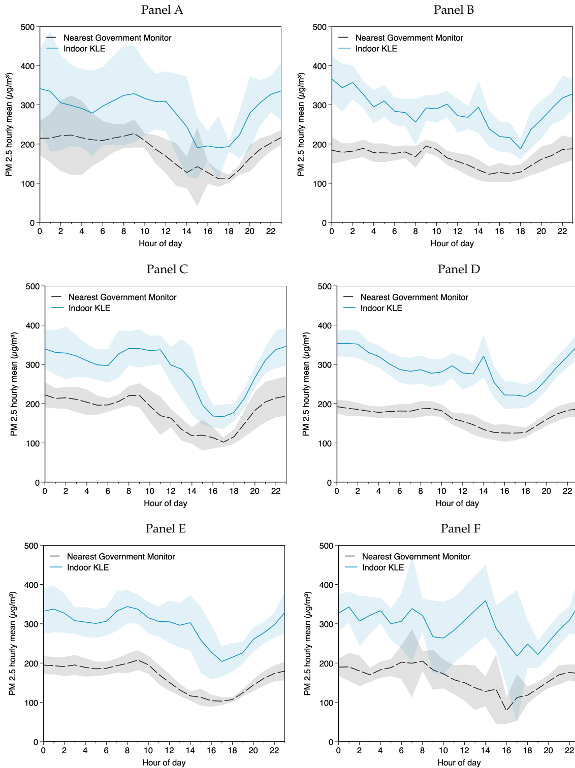
Figure A8C—Additional examples of indoor PM 2.5 patterns in high SES households
