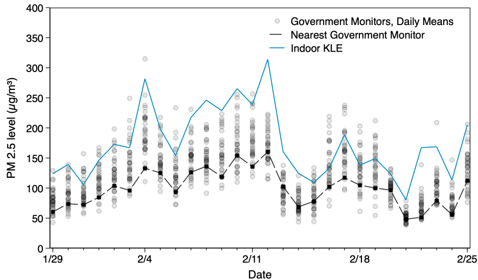
Figure A8B. Intra-city variation in ambient PM 2.5 measurements from government monitors
