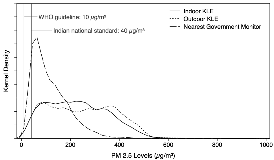
Figure A7. Indoor, outdoor, and nearest government monitor ambient PM 2.5 measurements at low SES households
