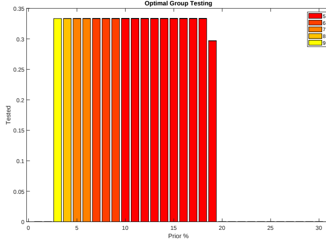
Figure 1: Optimal testing policy when pool tests of up to ten agents can be conducted; agents’ infection risks are uniformly distributed from 0% to 30%; the supply of tests is exactly enough to individually test 1 in 10 agents (hence, barely enough to test all agents with maximal grouping); and the planner’s preferences exhibit indifference to the quarantine decision for an agent of infection risk \frac{1}{15} \approx 6.67\% .
